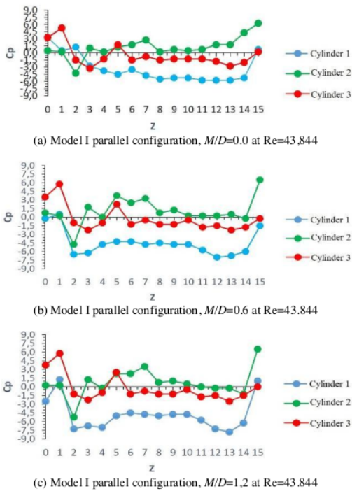
Figs. 4. Relationship of pressure coefficient ( C_p ) and the position of measurement points of cylinders 1, 2 and 3 at Re=43,844 , for three tandem square cylinder in model I parallel configuration (a) M/D=0.0 , (b) M/D=0.6 and (c) M/D=1.2
