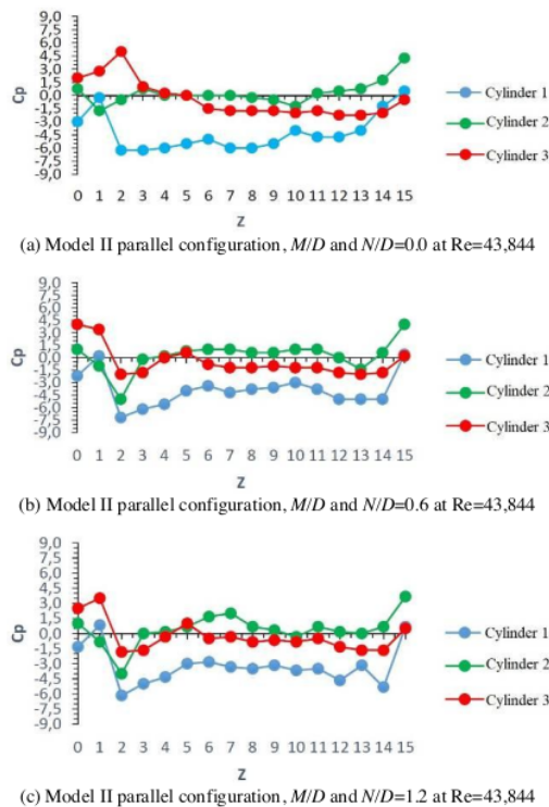
Figs. 5. Relationship of pressure coefficient ( C_p ) and the position of measurement points of cylinders 1, 2 and 3 at Re=43,844 , three tandem square cylinder in parallel configuration model II, (a) M/D and N/D=0.0 , (b) M/D and N/D=0.6 and (c) M/D and N/D=1.2
