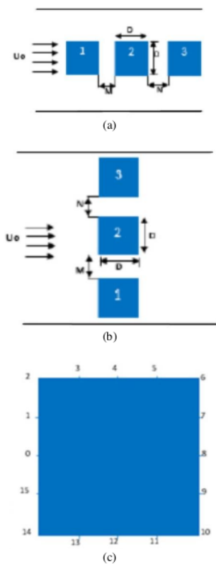
Figs. 1. Three square cylinders arranged in tandem in (a) serial and (b) parallel configuration and (c) taping position of each cylinder
