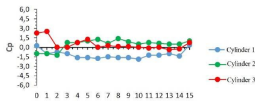
(a) Model II serial configuration, M/D and N/D=0.0 on Re=43,844
